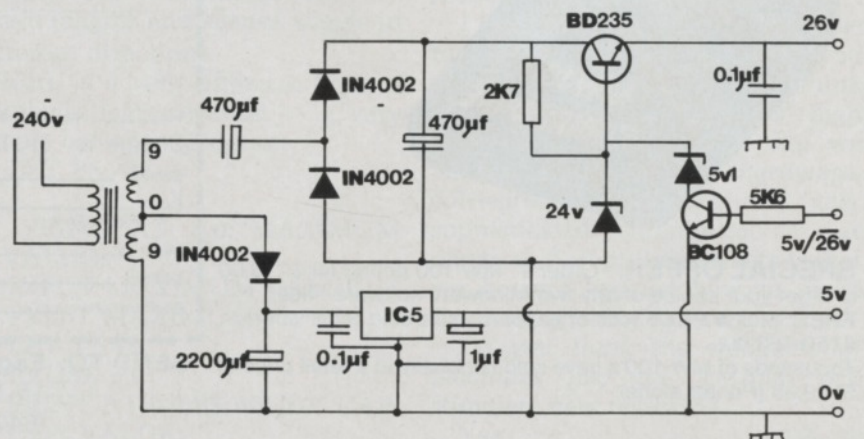
Figure 1: Driver circuit
